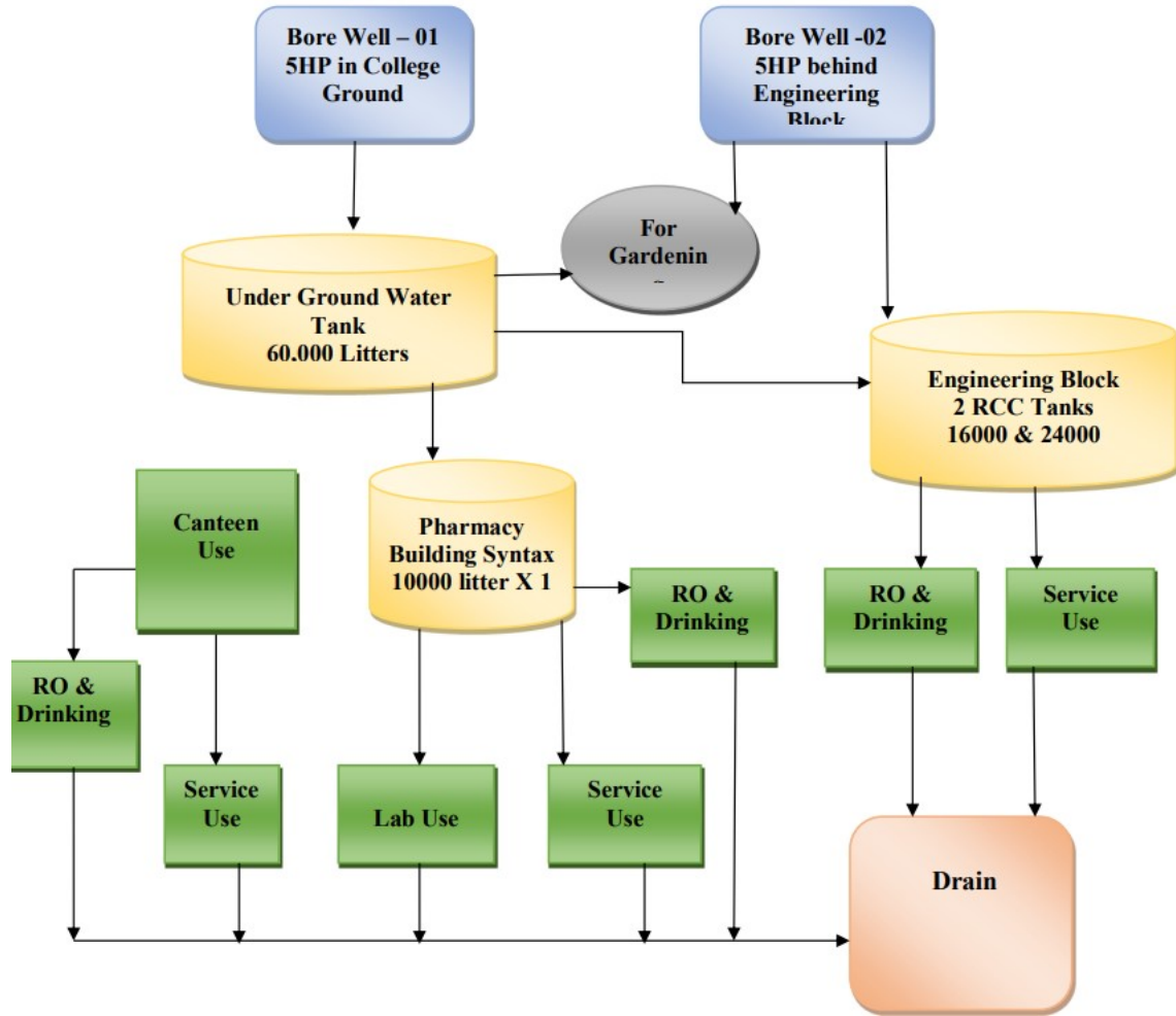
Water Flow Diagram of Institute
